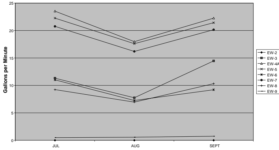
Monthly Average Pumping Rates for Extraction Wells -- 3Q08
