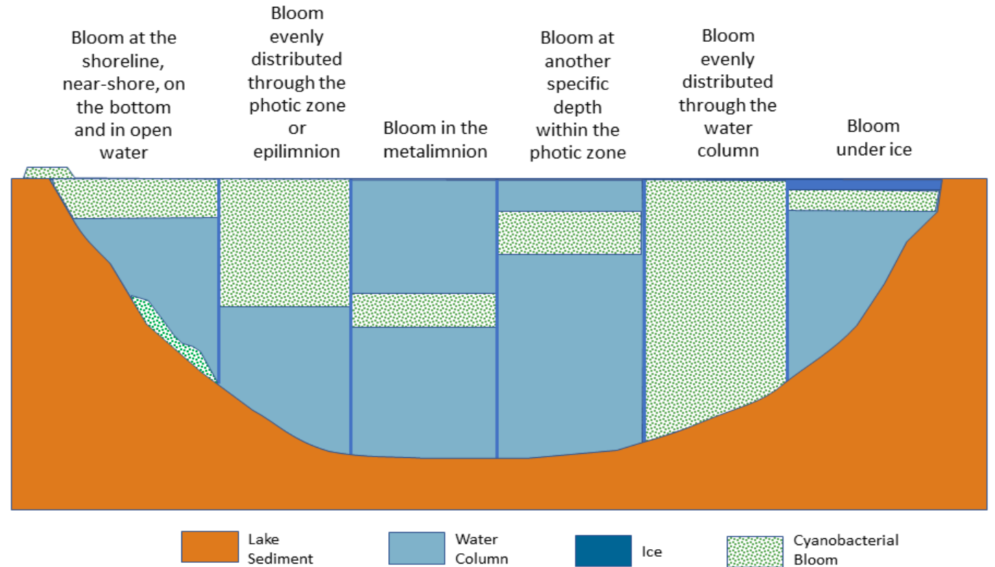
Fig. 4 – 1. Examples of cyanobacteria distribution in a lake or pond. Source: modified from Graham et al. 2008, used with permission.
