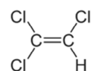
TCE ( C_2HCl_3 ) trichloroethene trichloroethylene
