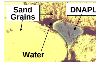
DNAPL Pore-Scale Distribution
