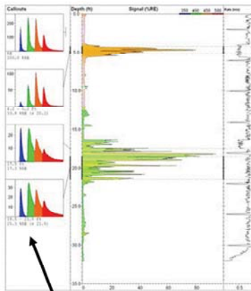
Waveform Indicates General Fuel Type
