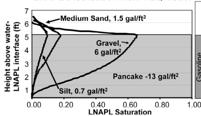
LNAPL Distribution from VEQ Model
