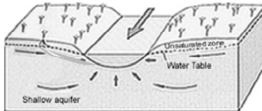
Image from U.S. Geological Survey
