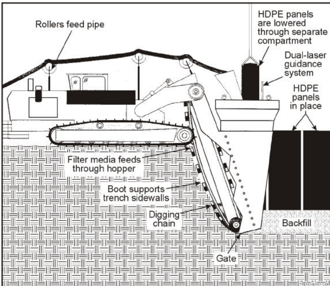
Figure 7-6. Continuous Trencher
