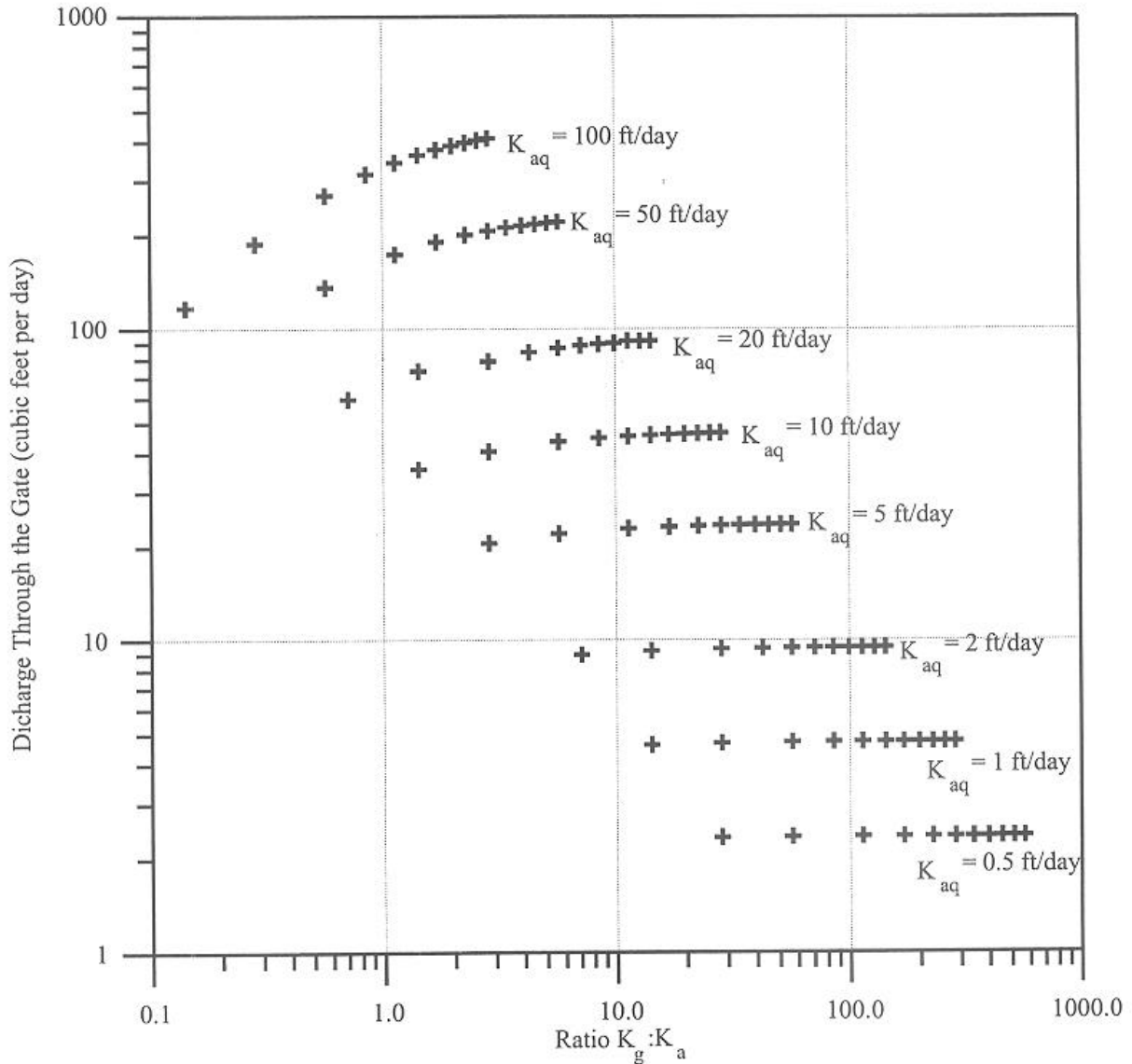
Figure C-5. Correlation Between Ratio of K_{cell} to K_{aquifer} Versus Discharge Through the Gate for a Homogeneous, One-Layer Scenario
