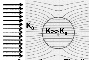
Groundwater Flowlines
