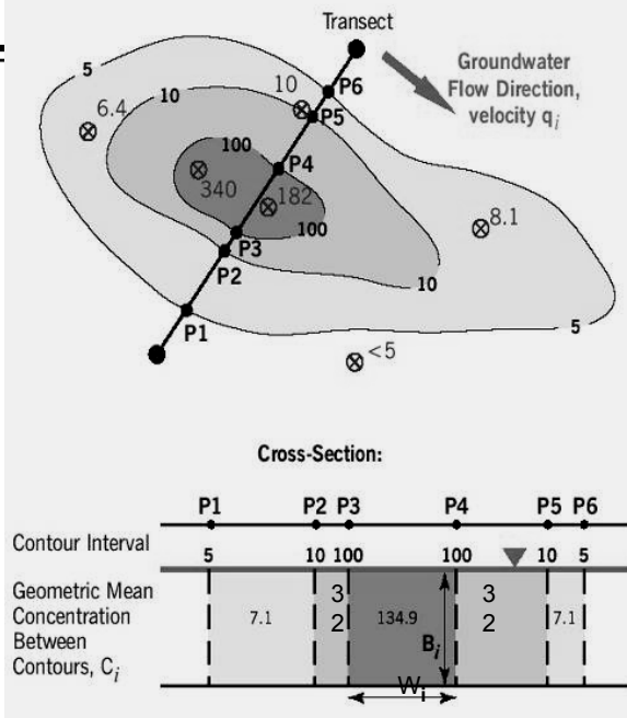
⊗ Single-Level Monitoring Well and Hypothetical Contaminant Concentration
