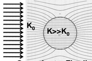
Groundwater Flowlines
