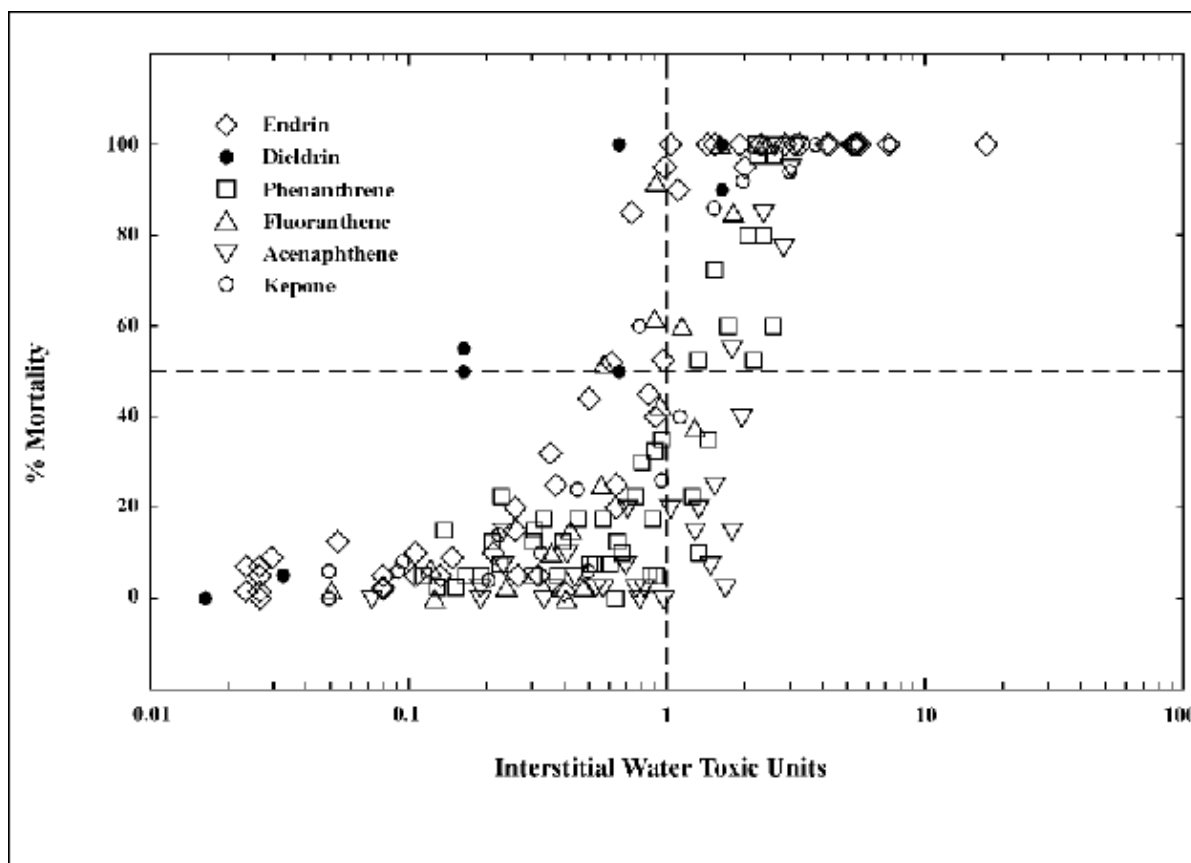
Figure 4-1. Percent mortalities of amphipods in sediments spiked with acenaphthene or phenanthrene (Swartz, 1991), endrin (Nebeker et al., 1989; Schuytema et al., 1989), or fluoranthene (Swartz et al., 1990; DeWitt et al., 1992), and midge in sediments spiked with dieldrin (Hoke et al., 1995) or kepone (Adams et al., 1985) relative to interstitial water units.
