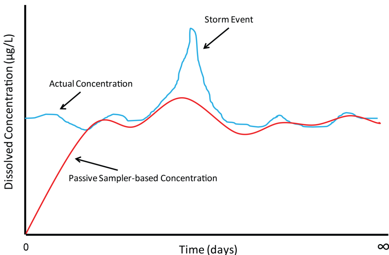
Figure 1. Conceptual diagram of the dissolved water column concentration of a hydrophobic contaminant shown as the actual concentration (blue line) and the passive sampler-based concentration (red line).
