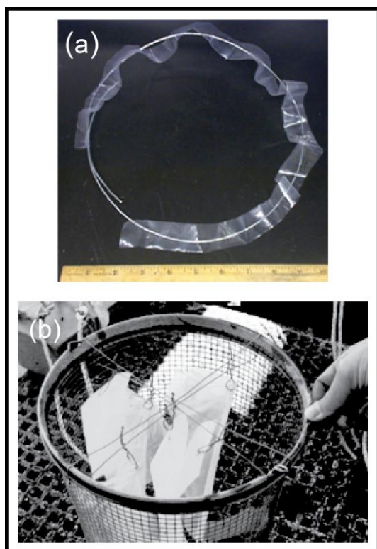
Figure 6. Passive samplers designed for water column deployments: (a) long strip of polyethylene on a stainless steel wire loop, and (b) polyethylene and polyoxymethylene strips fastened to the interior of a fish trap.
