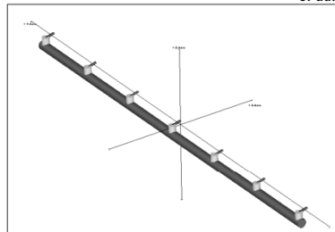
CorSpy visualization of an Unidirectional Multiport Diffuser
