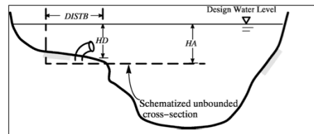
Schematizations for positively buoyant discharge
