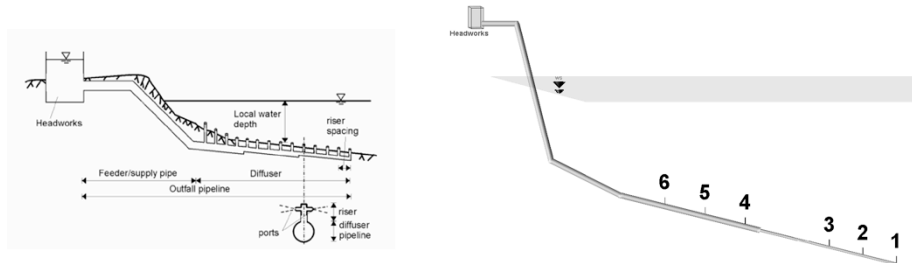
Schematic sketch (above) and CorHyd visualization (right) of a multiport diffuser outfall
