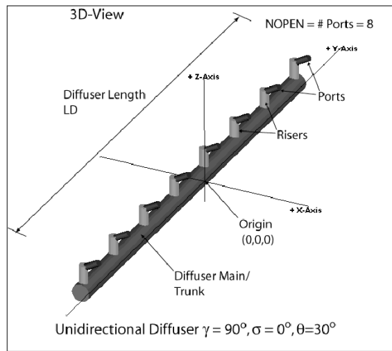
Multiport Diffuser Specification & Visualization In CorSpy
