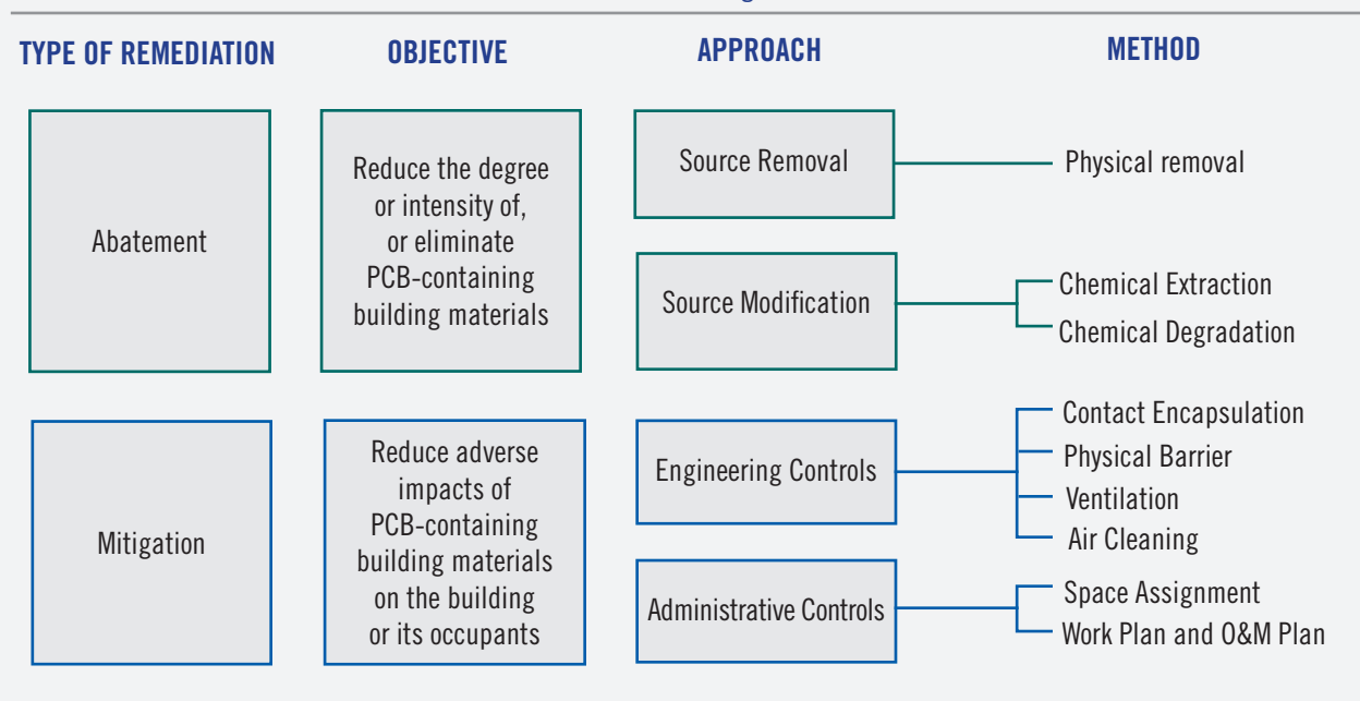
FIGURE 2.1 Framework for Methods to Remediate PCBs in Building Materials
