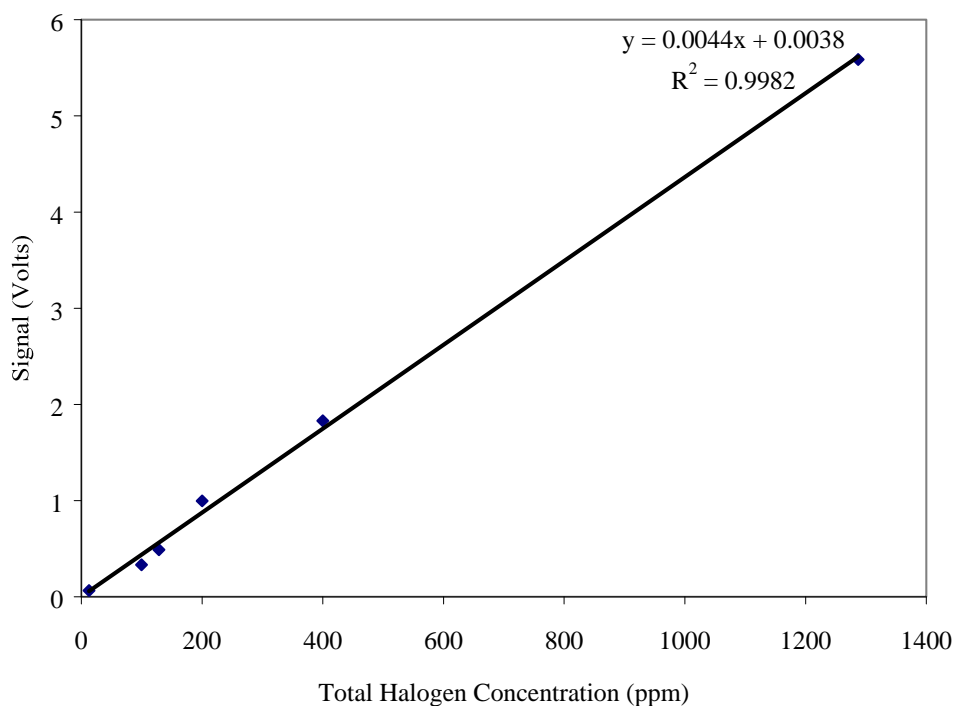
Figure 5. Correlation of XSD-MIP signal with TCE concentration
