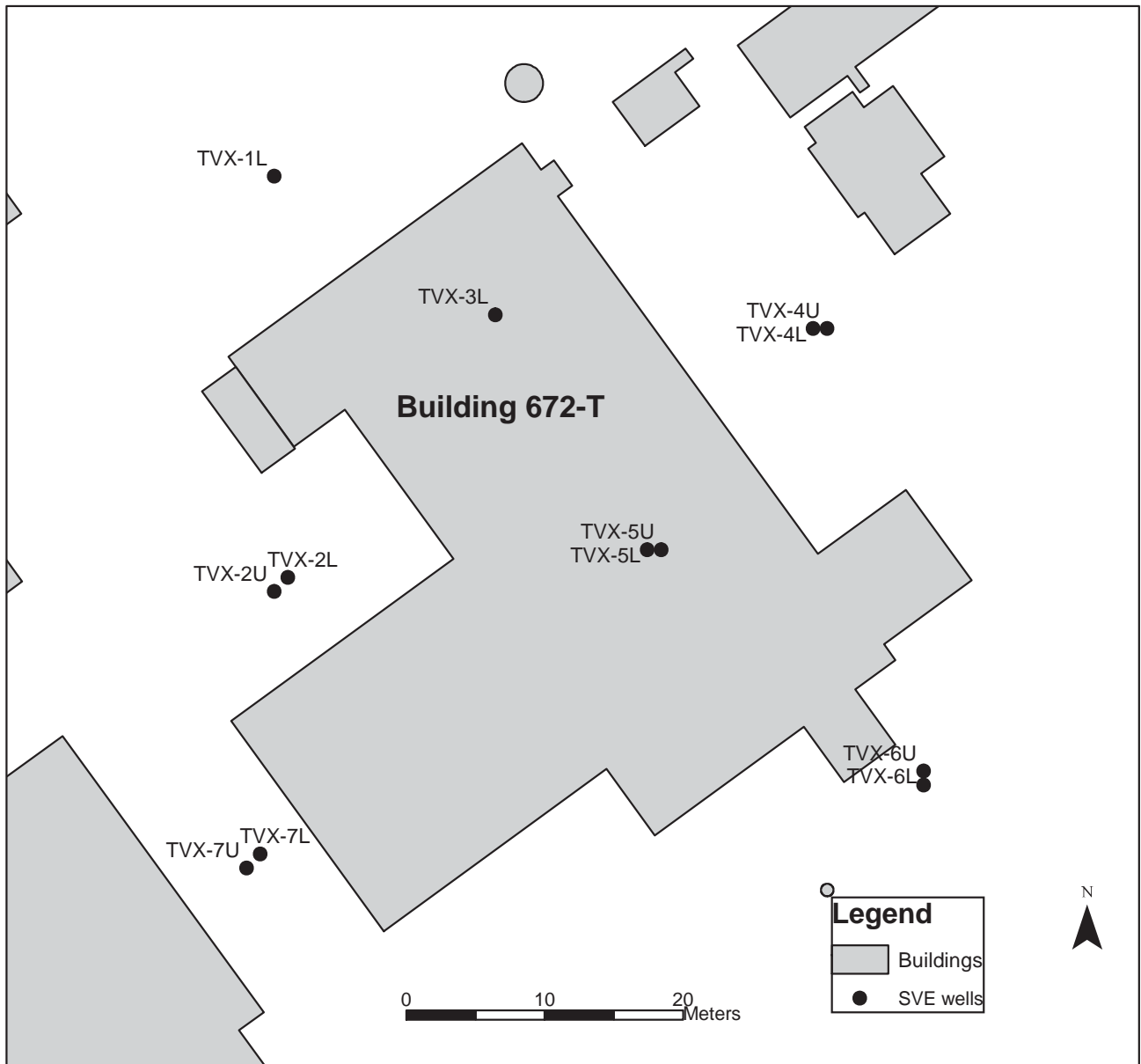
Figure 10: Soil Vapor Extraction Wells
