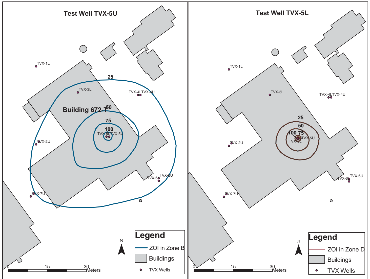
Figure 12: Contour Map of Vacuum during Baseline Test at TVX-5L and TVX-5U
