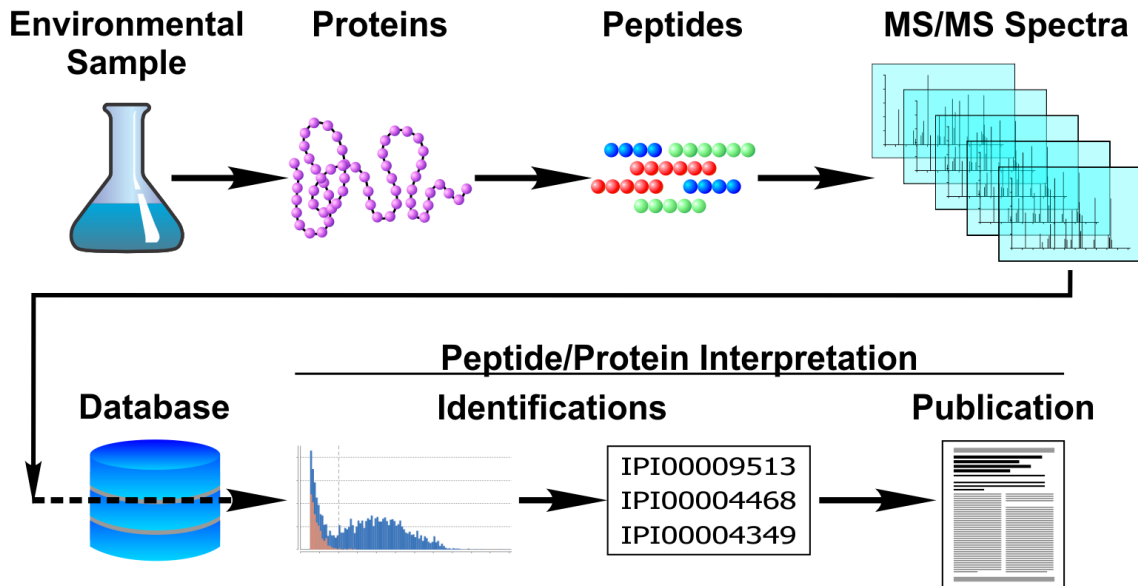
Figure 2.0-4. Metaproteomic Workflow for Environmental Samples
