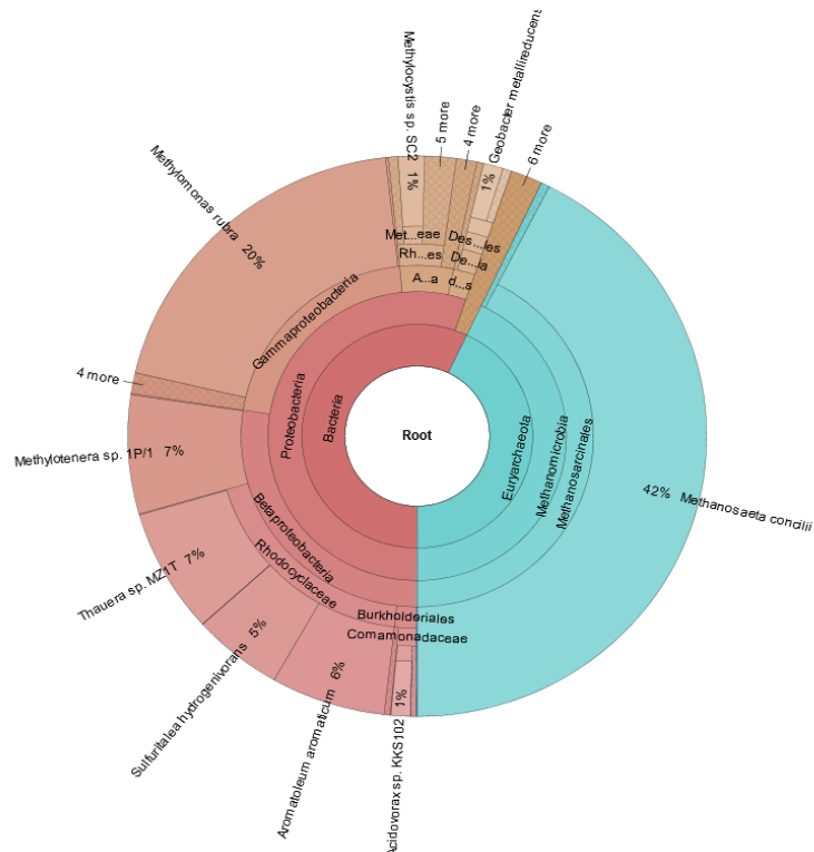
Figure D-12. Approximately Genus-level Depiction of Microbial Population for Sample 1327-MW-39 Collected during: A) Sampling Event 1 and B) Sampling Event 2
