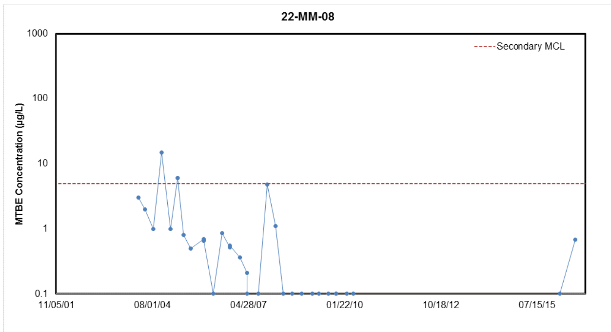
Figure C-2. MTBE Degradation Trend in Well 22-MM-08 at the 22 MCX Gas Station Site
