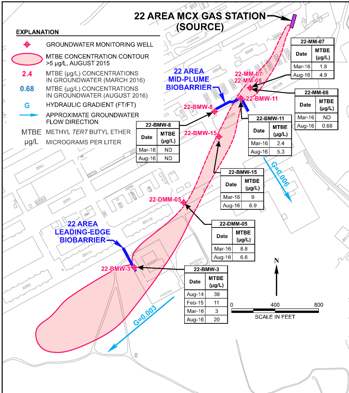
Figure 4-3. MTBE Concentrations in Groundwater at the 22 Area MCX Gas Station Site (August/September 2014, February 2015, March 2016 and August 2015)
