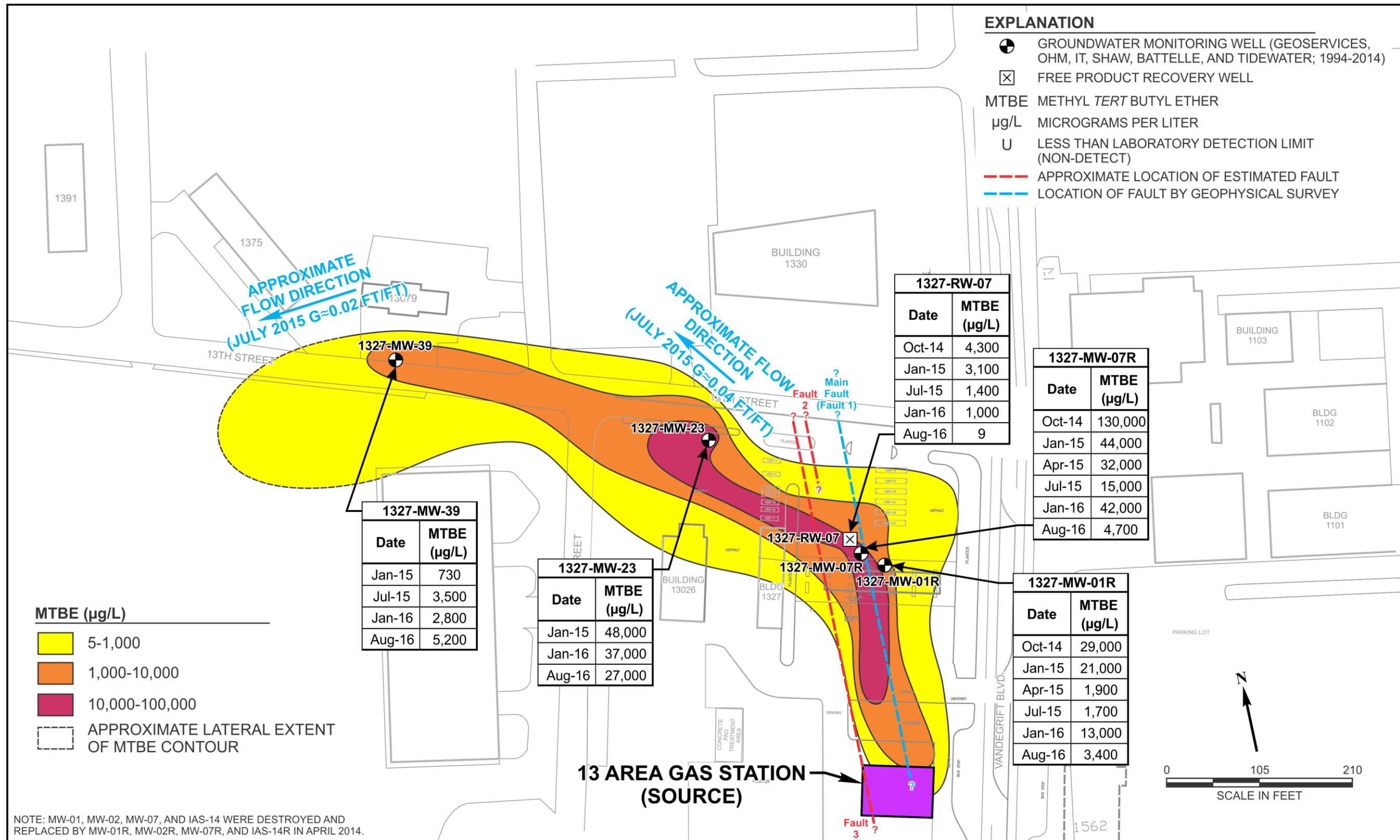
Figure 4-6. MTBE Concentrations from 2014 through 2016 at 13 Area Gas Station MCB Camp Pendleton
