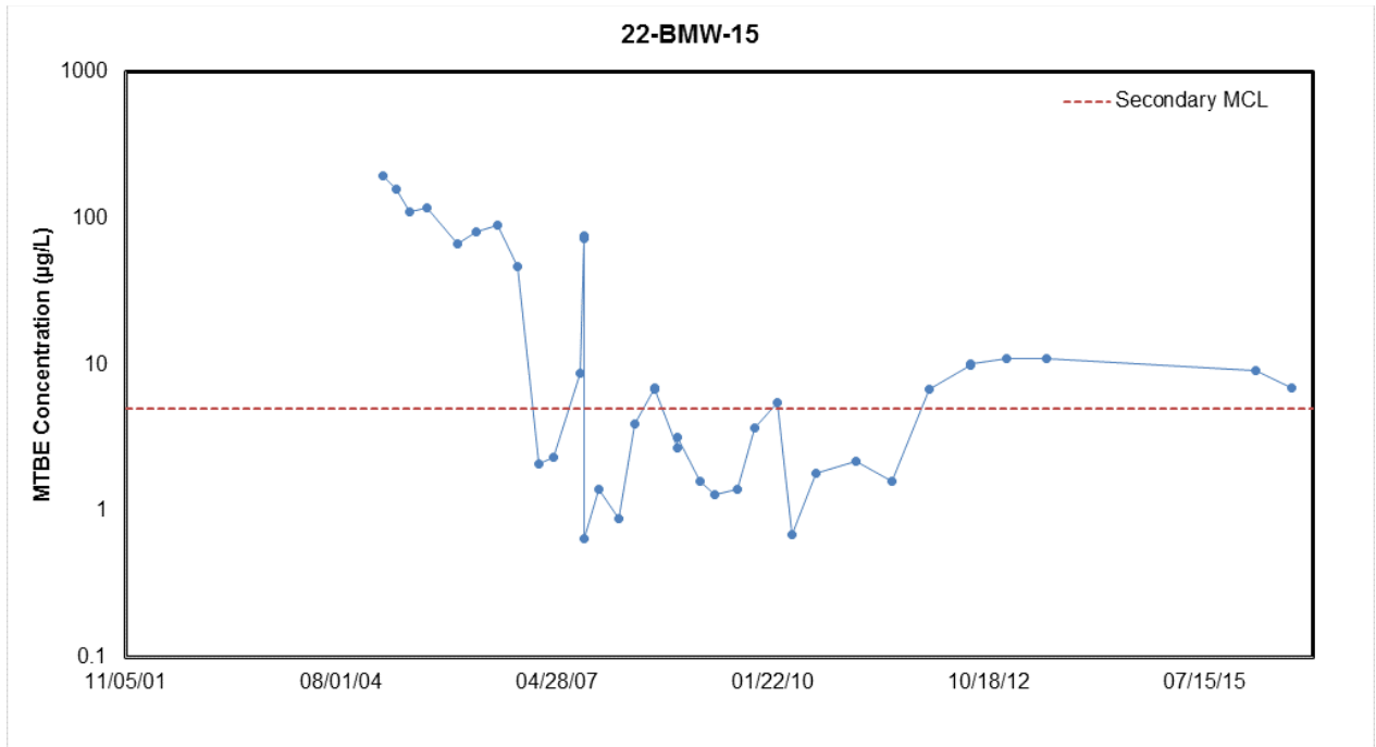
Figure C-5. MTBE Degradation Trend in Well 22-BMW-15 at the 22 MCX Gas Station Site
