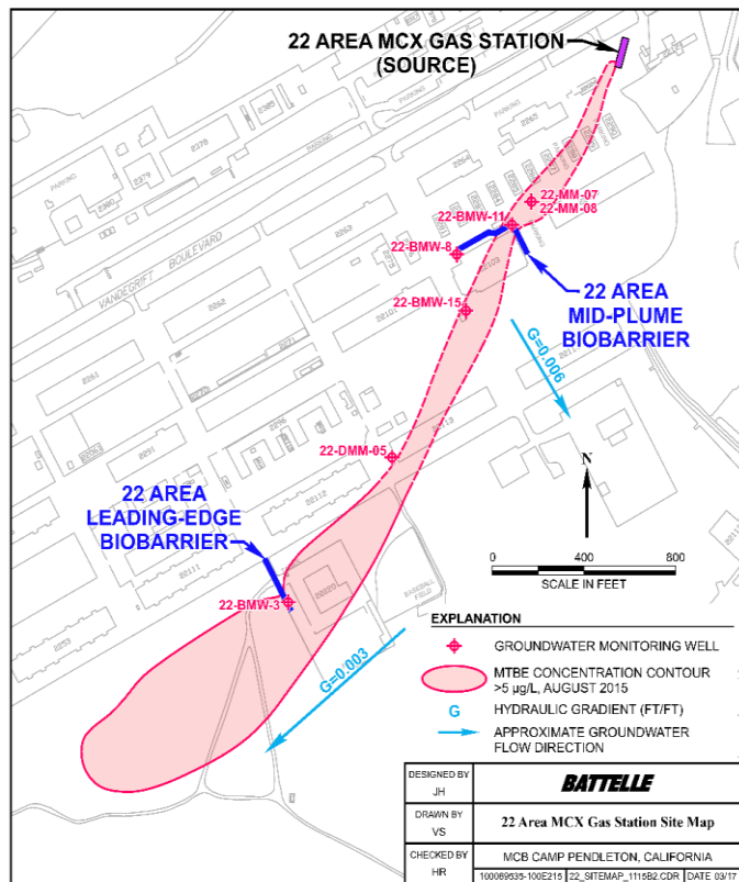
Figure 1-1. 22 MCX Gas Station Site Map
