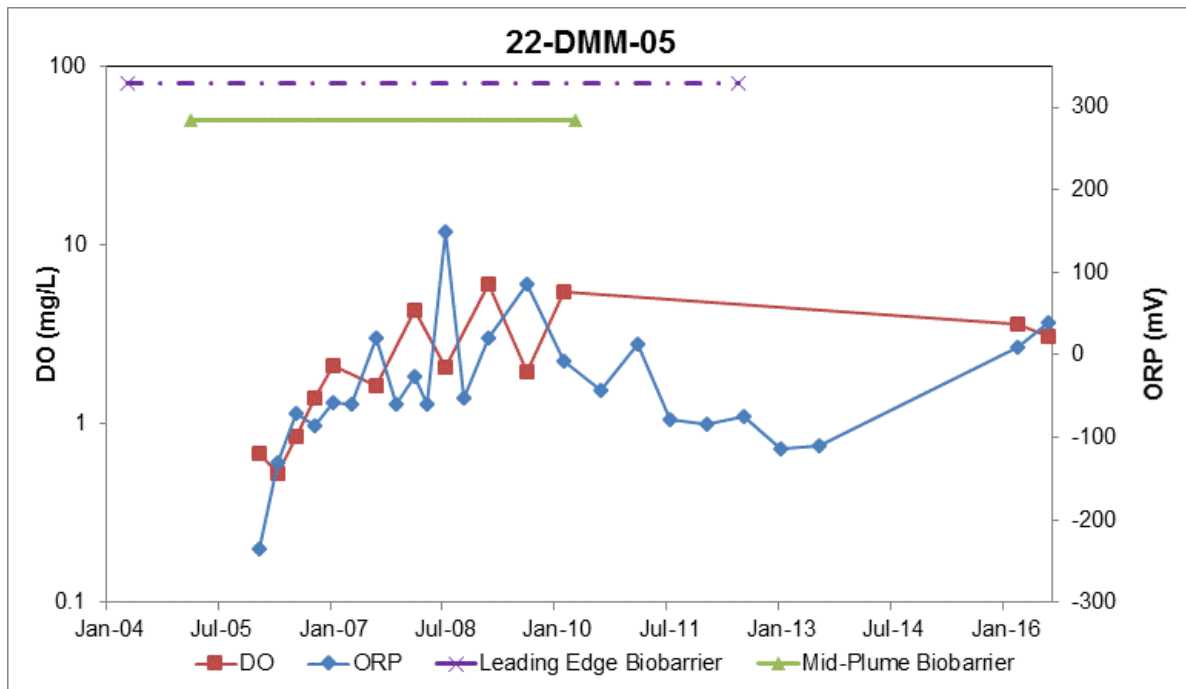
Figure C-13. DO and ORP Trend in Well 22-DMM-05 at the 22 MCX Gas Station Site
