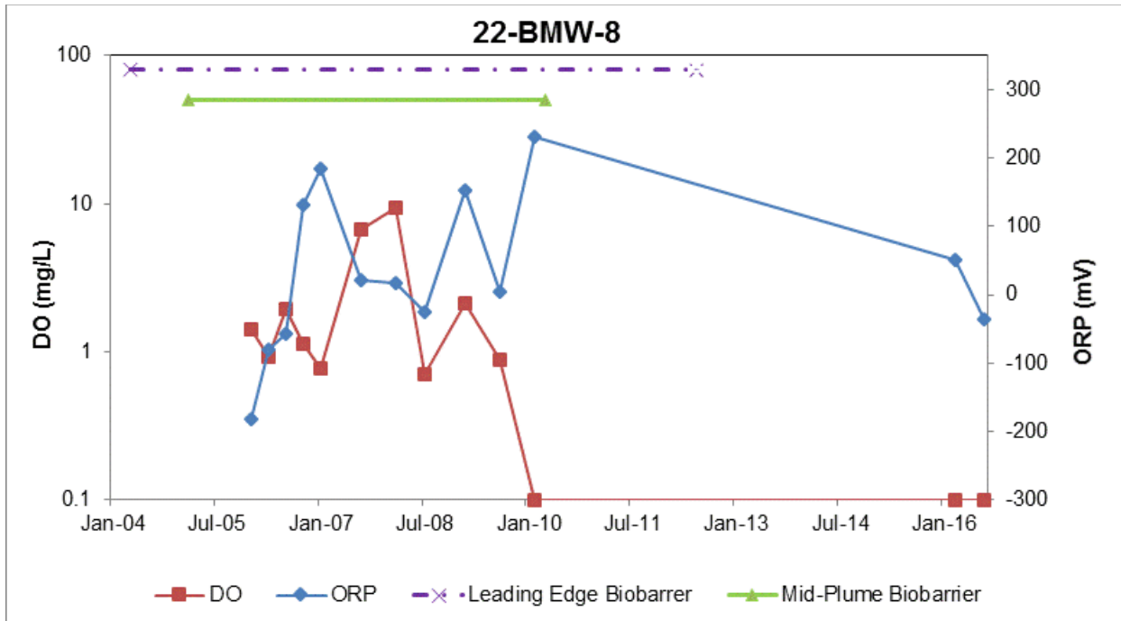
Figure C-11. DO and ORP Trend in Well 22-BMW-8 at the 22 MCX Gas Station Site
