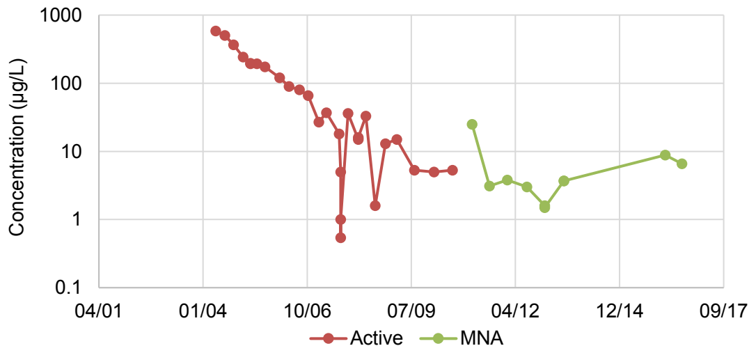
Figure 5-3. Trends of MTBE Concentration over Time for a Representative Well (22-DMM-05) at 22 MCX Gas Station Evaluated with Mann Kendall Analysis
