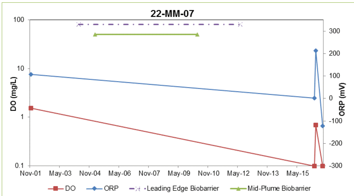
Figure C-8. DO and ORP Trend in Well 22-MM-07 at the 22 MCX Gas Station Site
