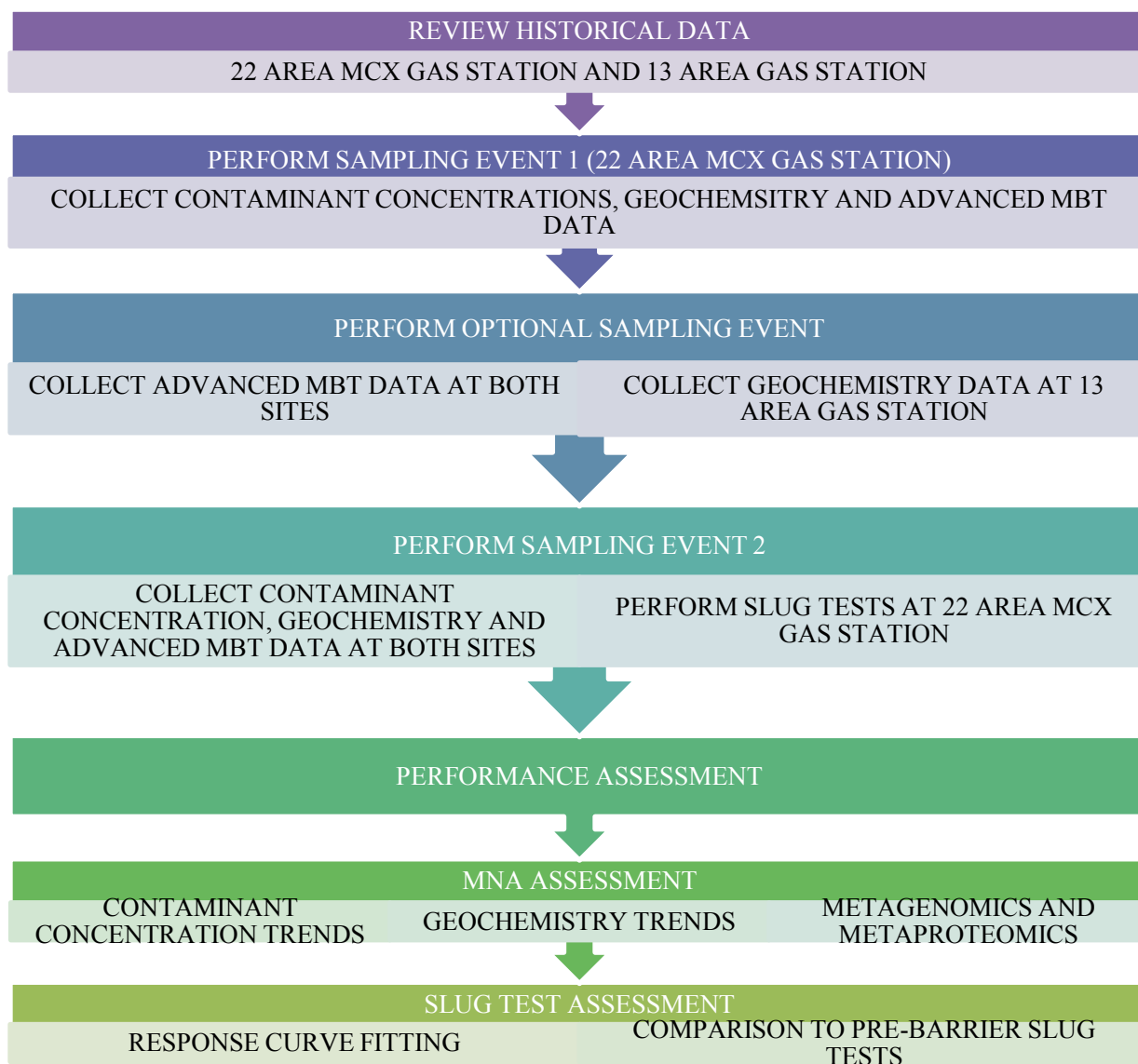
Figure 5-1. Conceptual Design for the Demonstration
