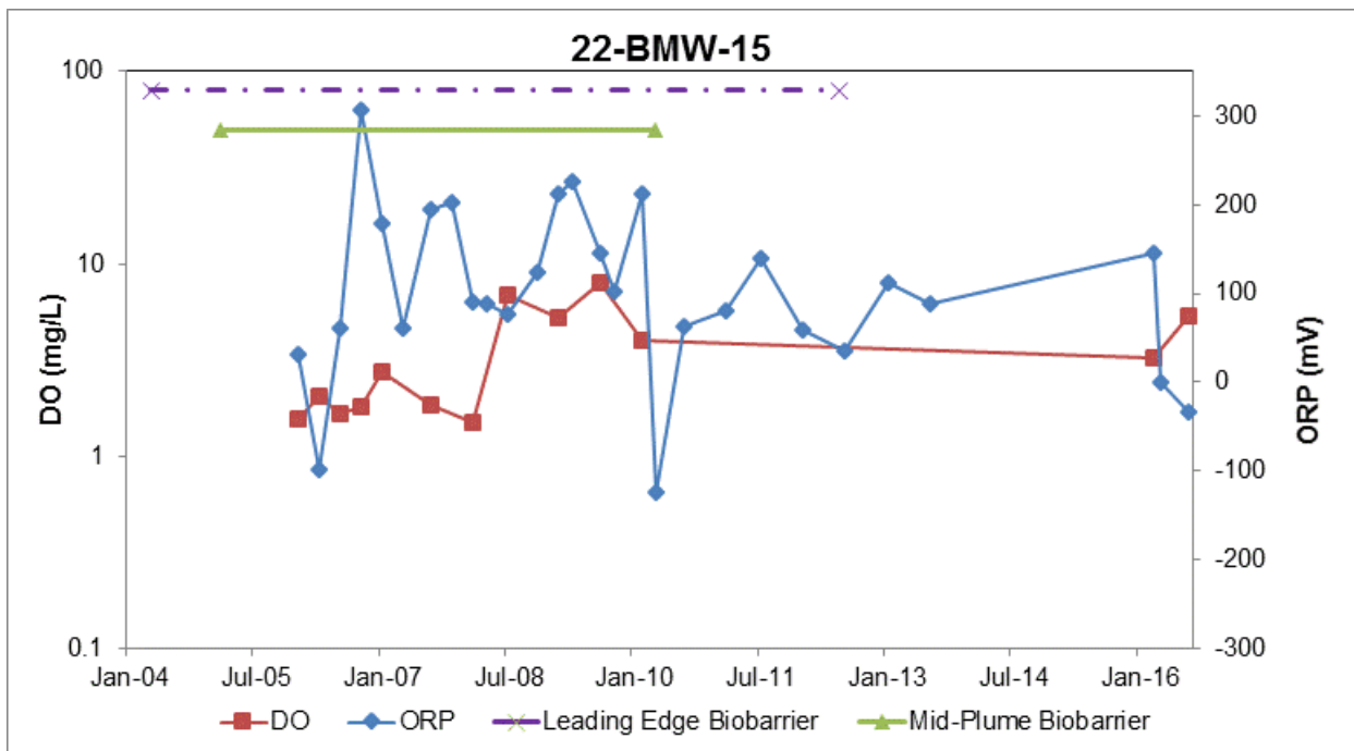
Figure C-12. DO and ORP Trend in Well 22-BMW-15 at the 22 MCX Gas Station Site
