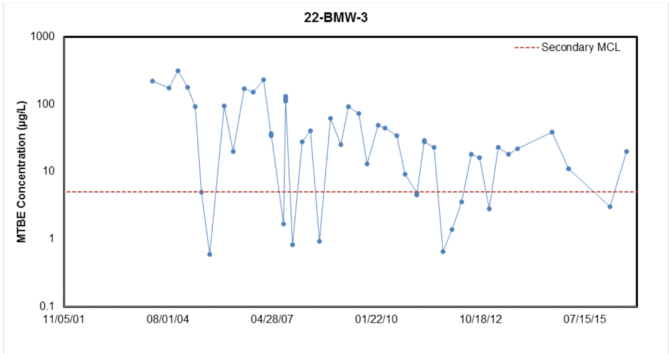
Figure C-7. MTBE Degradation Trend in Well 22-BMW-3 at the 22 MCX Gas Station Site
