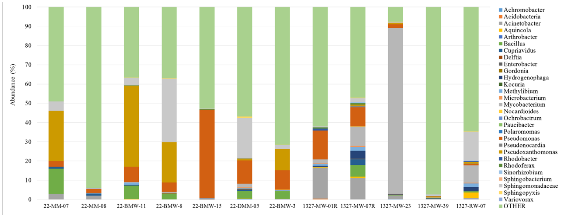
Figure D-18. Percentage Abundance of Microbial MTBE and TBA Degrading Microorganisms on Genus Level Detected in Samples Collected from 22 Area MCX Gas Station and 13 Area Camp Pendleton Site during Sampling Event 2
