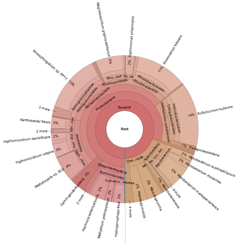
Figure D-9. Approximately Genus-level Depiction of Microbial Population for Sample 1327-RW-07 Collected during: A) Sampling Event 1 and B) Sampling Event 2
