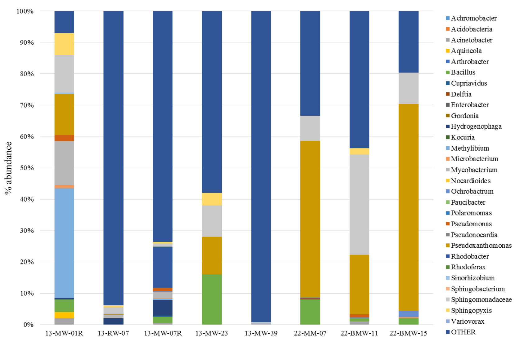
Figure D-16. Percentage Abundance of Microbial MTBE and TBA Degrading Microorganisms on Genus Level Detected in Samples Collected from 22 Area MCX Gas Station and 13 Area Camp Pendleton Site during Optional Sampling Event
