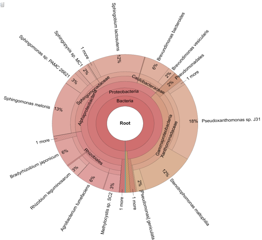
Figure D-3. Approximately Genus-level Depiction of Microbial Population for Sample 22-BMW-11 Collected during: A) Sampling Event 1 and B) Sampling Event 2
