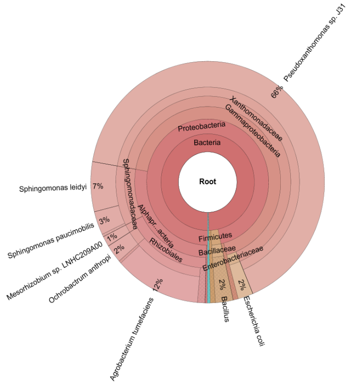
Figure D-5. Approximately Genus-level Depiction of Microbial Population for Sample 22-BMW-15 Collected during: A) Sampling Event 1 and B) Sampling Event 2
