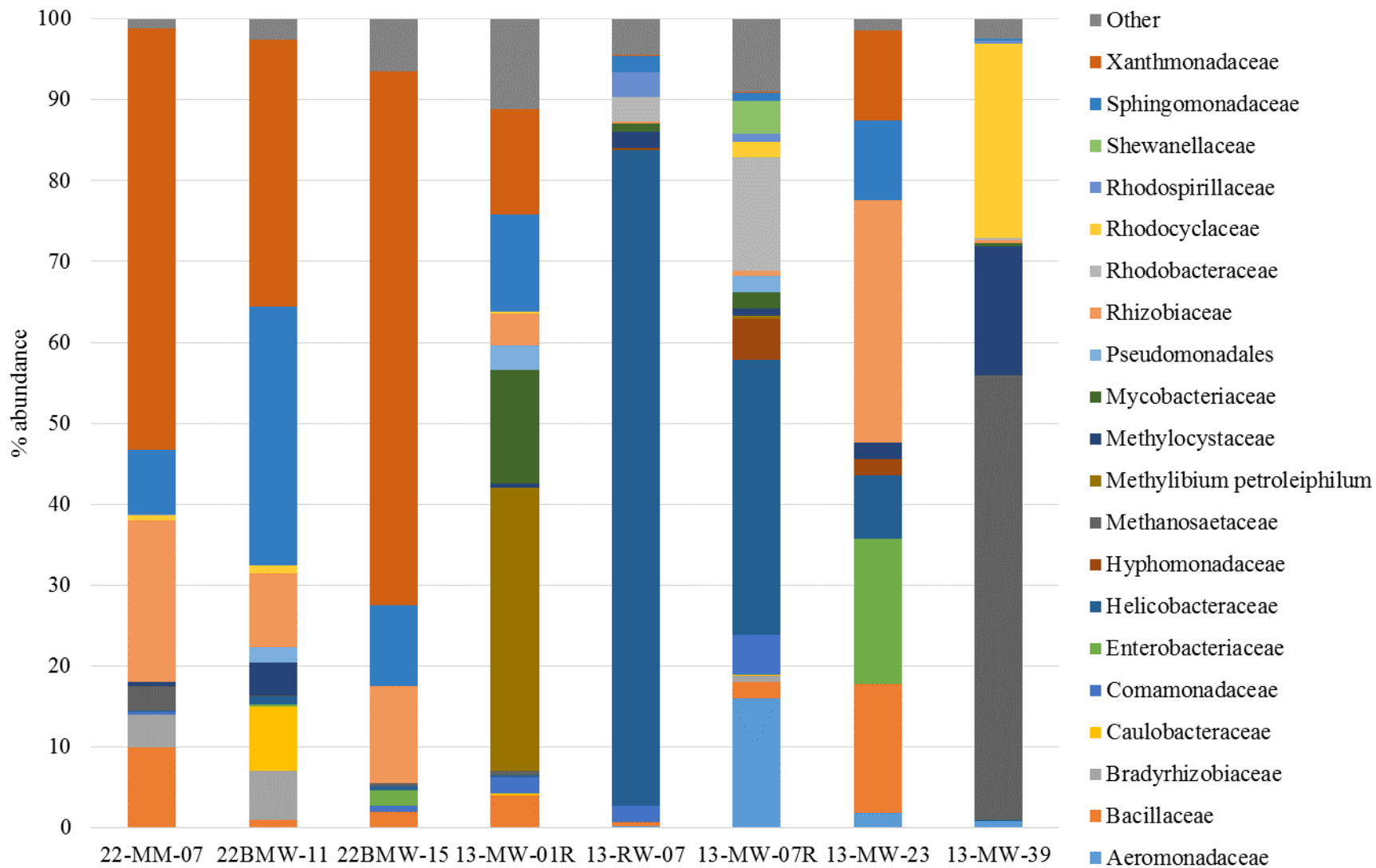
Figure D-15. Percentage Abundance of Microbial Families Found in Samples Collected from 22 Area MCX Gas Station and 13 Area Camp Pendleton Site during Optional Sampling Event
