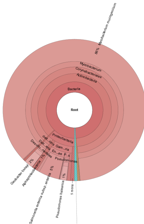
Figure D-11. Approximately Genus-level Depiction of Microbial Population for Sample 1327-MW-23 Collected during: A) Sampling Event 1 and B) Sampling Event 2
