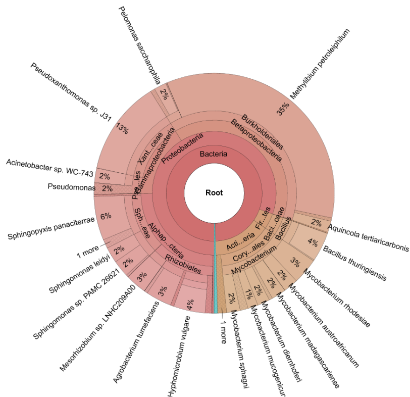
Figure 5-7. Krona Plot Illustrating Abundance of Microorganisms in the 1327-MW-01R Sample Collected in the Leading Edge of the Plume at the 13 Area Gas Station
