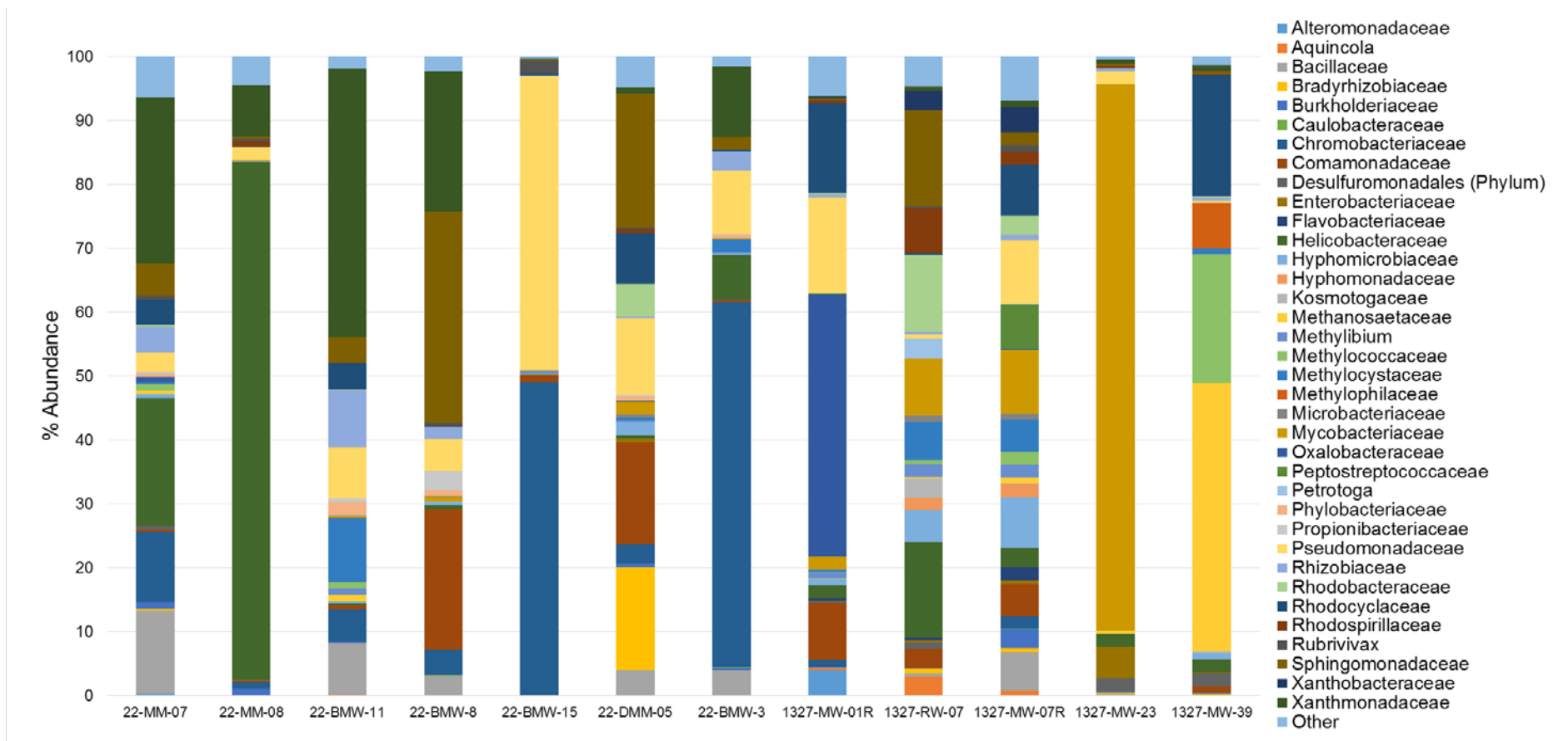
Figure D-17. Percentage Abundance of Microbial Families Found in Samples Collected from 22 Area MCX Gas Station and 13 Area Camp Pendleton Site during Sampling Event 2
