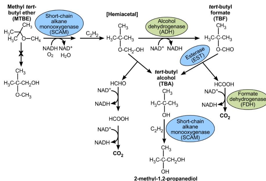
Figure 2.0-2. Initial Reactions and Corresponding Enzymes Determined in Cometabolic Degradation of MTBE by Propane-Grown Mycobacterium austroafricanum JOB (Smith, O'Reilly et al. 2003; Nava, Morales et al. 2007)
