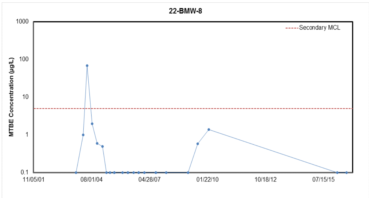
Figure C-4. MTBE Degradation Trend in Well 22-BMW-8 at the 22 MCX Gas Station Site
