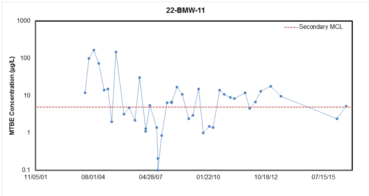
Figure C-3. MTBE Degradation Trend in Well 22-BMW-11 at the 22 MCX Gas Station Site
