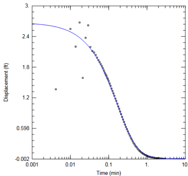
Figure 5-9. Response Curve for the Slug-out Test 3 for 22-MM-08 Where Equilibrium was Reached after Seven Minutes
