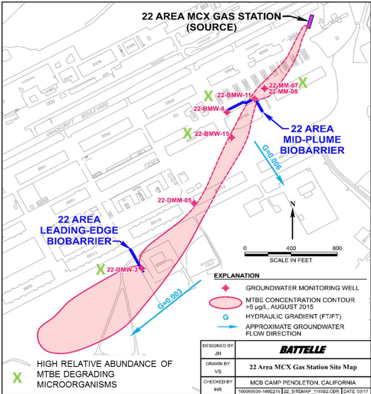
Figure 6-1. Location of Wells with High Percentage Relative Abundance of MTBE Degrading Microbial Species Detected during Sampling Events 1 and 2 at 22 Area MCX Gas Station
