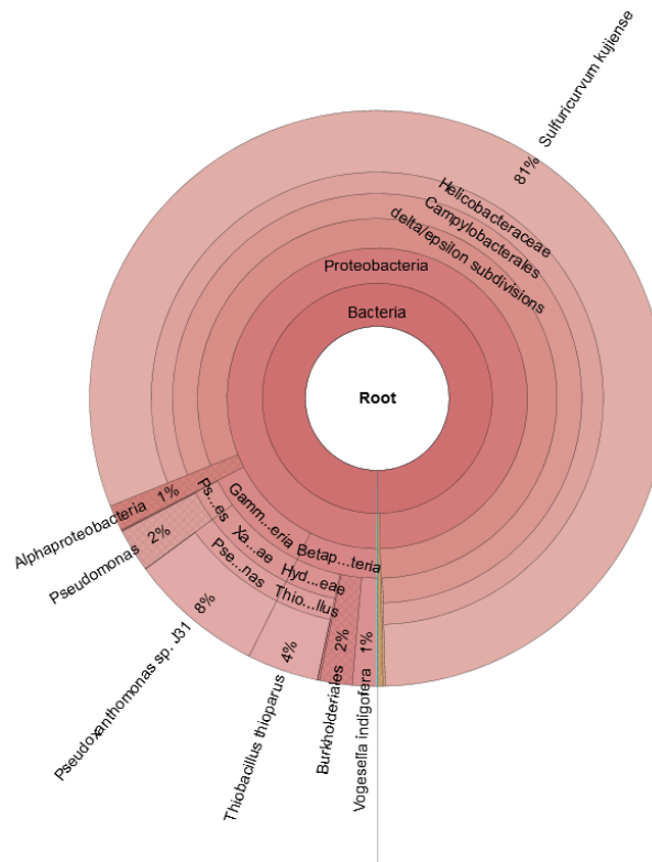
Figure D-2. Approximately Genus-level Depiction of Microbial Population for Sample 22-DMM-08 Collected during: A) Sampling Event 1 and B) Sampling Event 2
