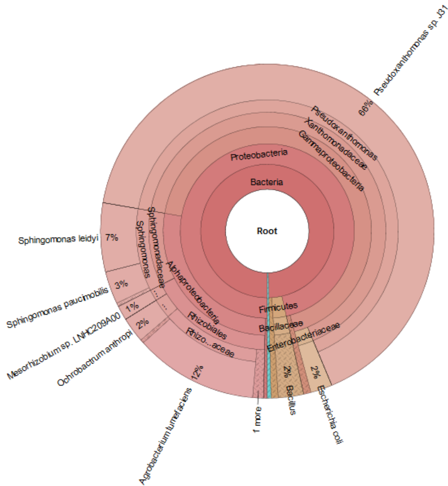
Figure 5-5. Krona Plot Illustrating Abundance of Microorganisms in the 22-BMW-15 Sample Collected in Between Biobarriers at the 22 Area MCX Gas Station
