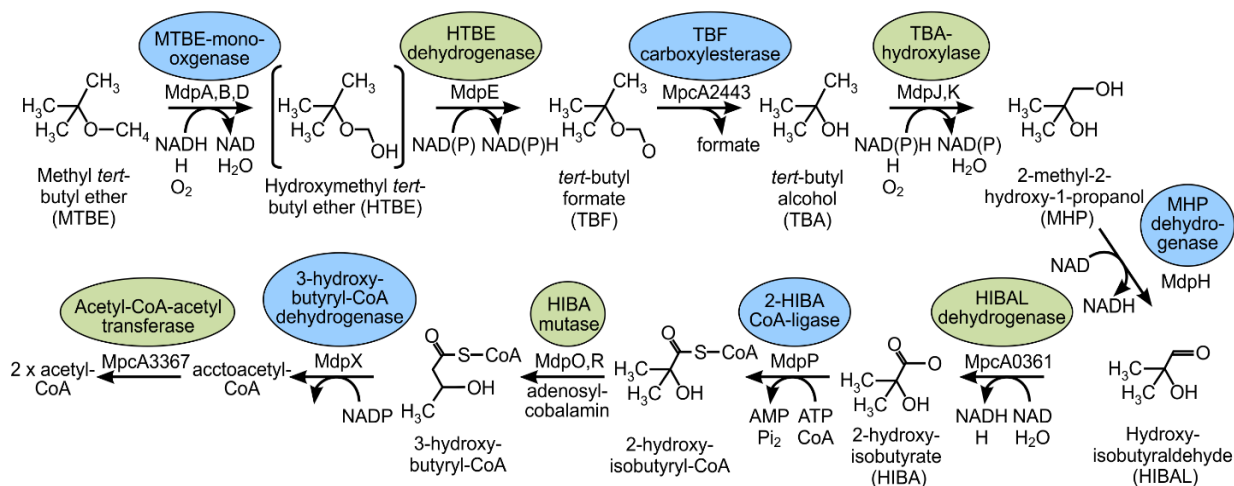
Figure 2.0-1. Peptides Involved in Degradation of Gasoline and Aromatic Compounds in M. petroleiphilum PM1(Hristova, Gebreyesus et al. 2003; Schmidt, Battaglia et al. 2008)
