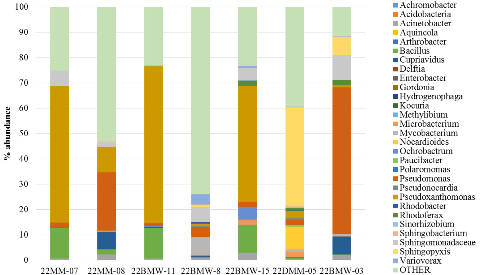
Figure D-14. Percentage Abundance of Microbial MTBE and TBA Degrading Microorganisms on Genus Level Detected in Samples Collected from 22 Area MCX Gas Station Site during Sampling Event 1
