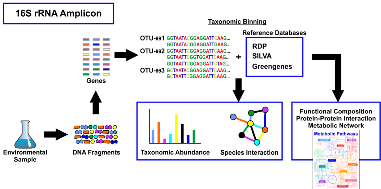
Figure 2.0-3. Metagenomic Workflow for Environmental Samples
