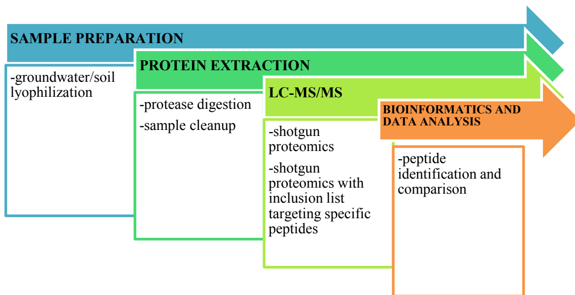
Figure 5-2. Steps Involved in Proteomic Analysis of Groundwater Samples
