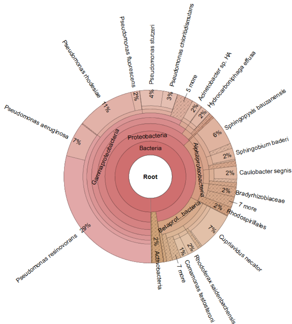
Figure 5-6. Krona Plot Illustrating Abundance of Microorganisms in the 22-BMW-3 Sample Collected in the Leading Edge of the Plume at the 22 Area MCX Gas Station
