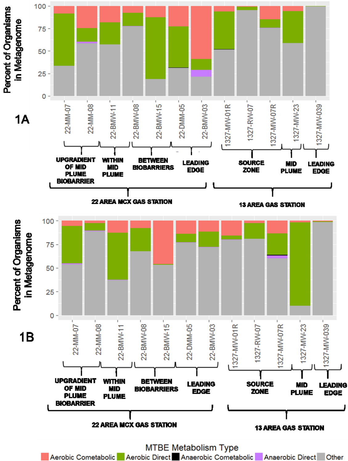
Figure 5-4. Percent Abundance of Microorganisms in Samples from the 22 Area MCX Gas Station and the 13 Area Gas Station where 1A is the First Sampling Event and 1B is the Second Sampling Event. MTBE-degrading Microorganisms were Categorized Depending on Aerobic/Anaerobic and Direct versus Cometabolic Degradation.
