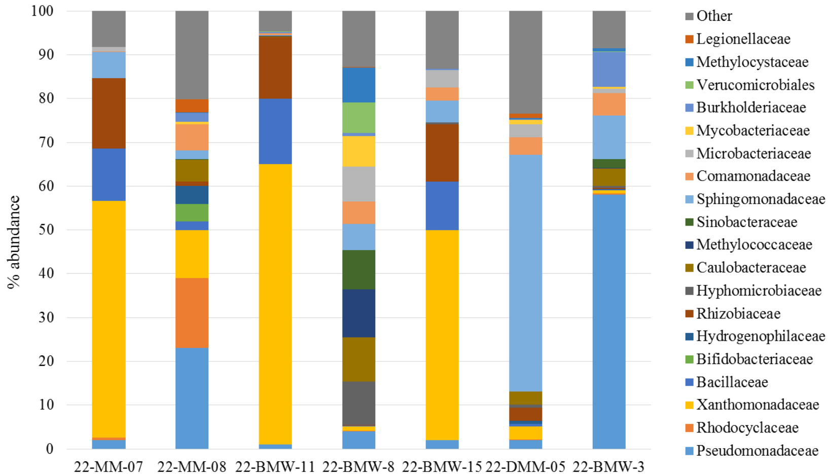
Figure D-13. Percentage Abundance of Microbial Families Found in Samples Collected from 22 Area MCX Gas Station Site during Sampling Event 1
