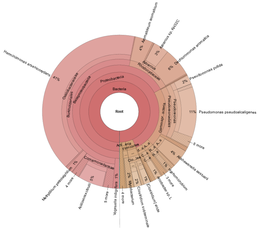
Figure D-8. Approximately Genus-level Depiction of Microbial Population for Sample 1327-MW-01R Collected during: A) Sampling Event 1 and B) Sampling Event 2
