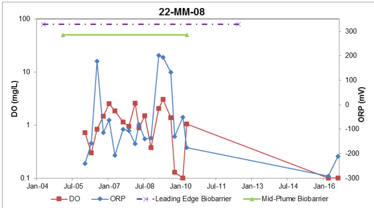
Figure C-9. DO and ORP Trend in Well 22-MM-08 at the 22 MCX Gas Station Site
