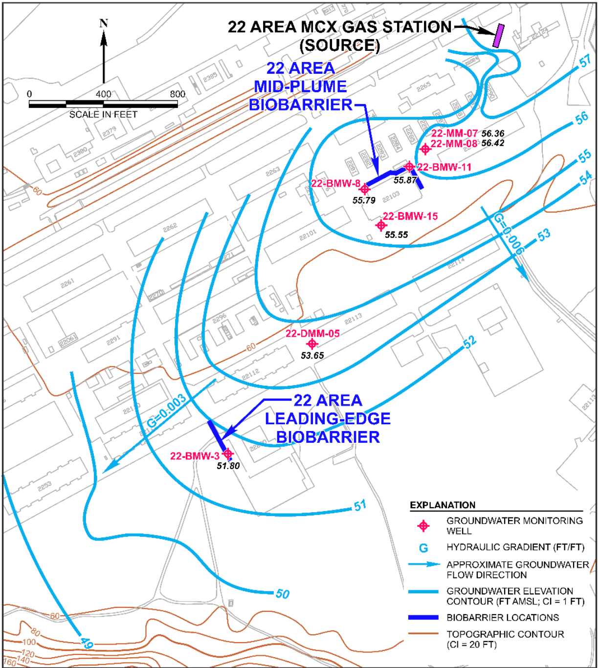
Figure 4-4. Elevation Contours, 22 Area MCX Gas Station Site, July 2015
