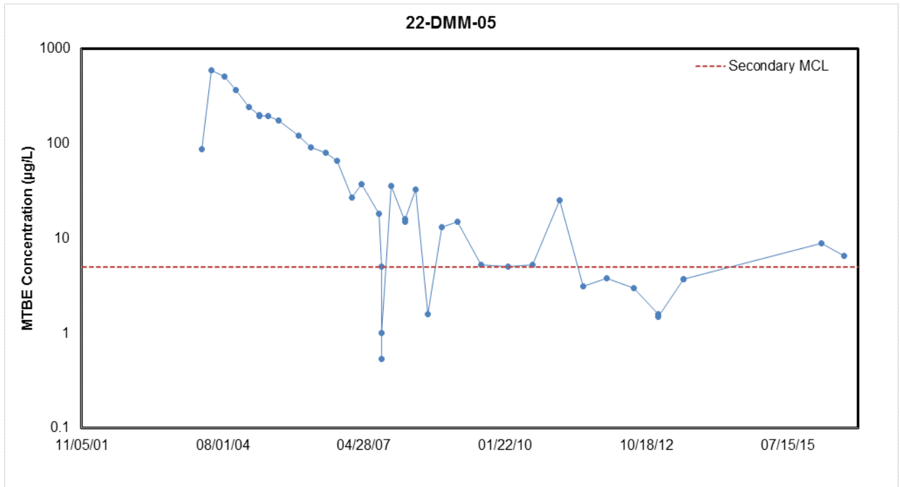
Figure C-6. MTBE Degradation Trend in Well 22-DMM-05 at the 22 MCX Gas Station Site
