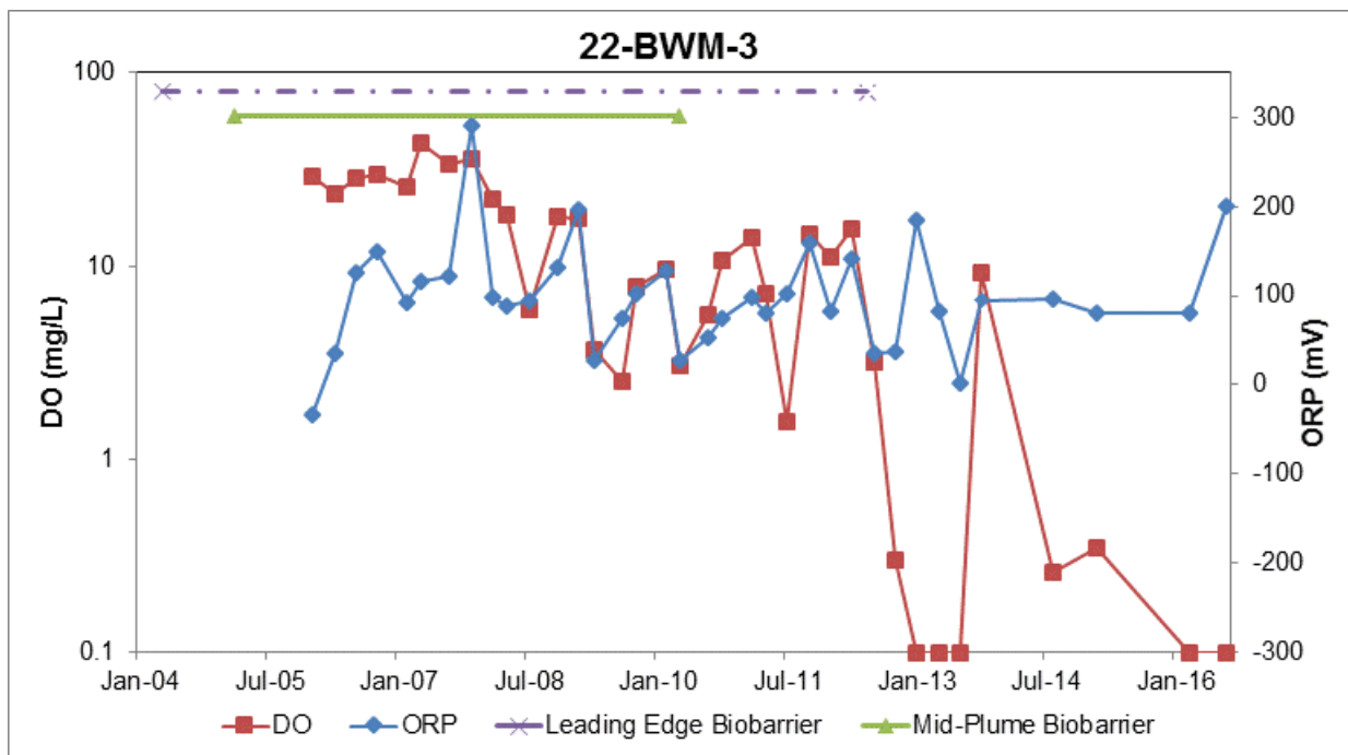
Figure C-14. DO and ORP Trend in Well 22-BMW-3 at the 22 MCX Gas Station Site
