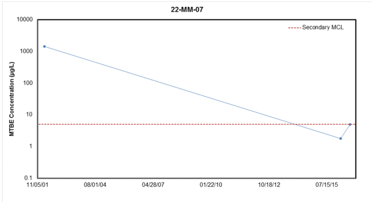
Figure C-1. MTBE Degradation Trend in Well 22-MM-07 at the 22 MCX Gas Station Site
