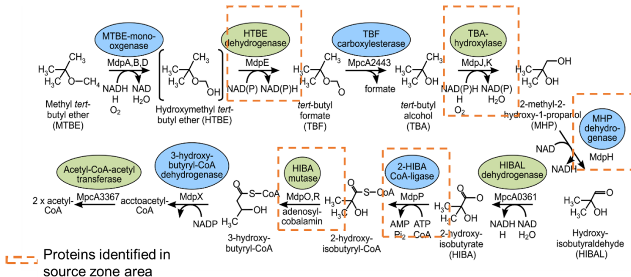
Figure 5-8. Proteins Involved in MTBE Degradation of M. petroleiphilum PM1 (Hristova, Gebreyesus et al. 2003; Schmidt, Battaglia et al. 2008)
