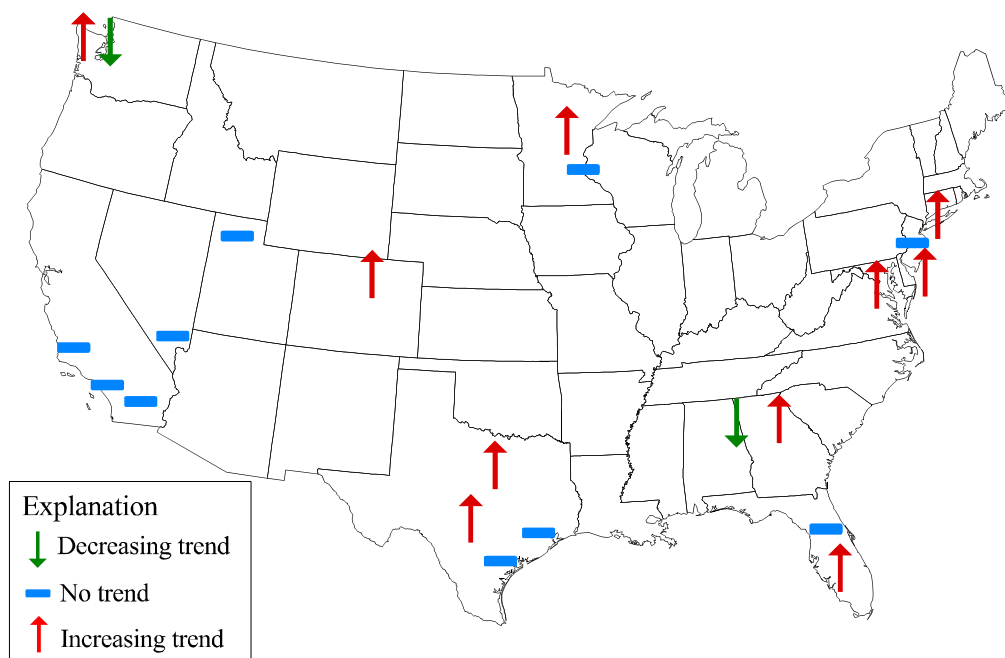
Figure 4-7. PAH Trends Throughout the United States Using Sediment Core Data from 1970 to Top of Core.
