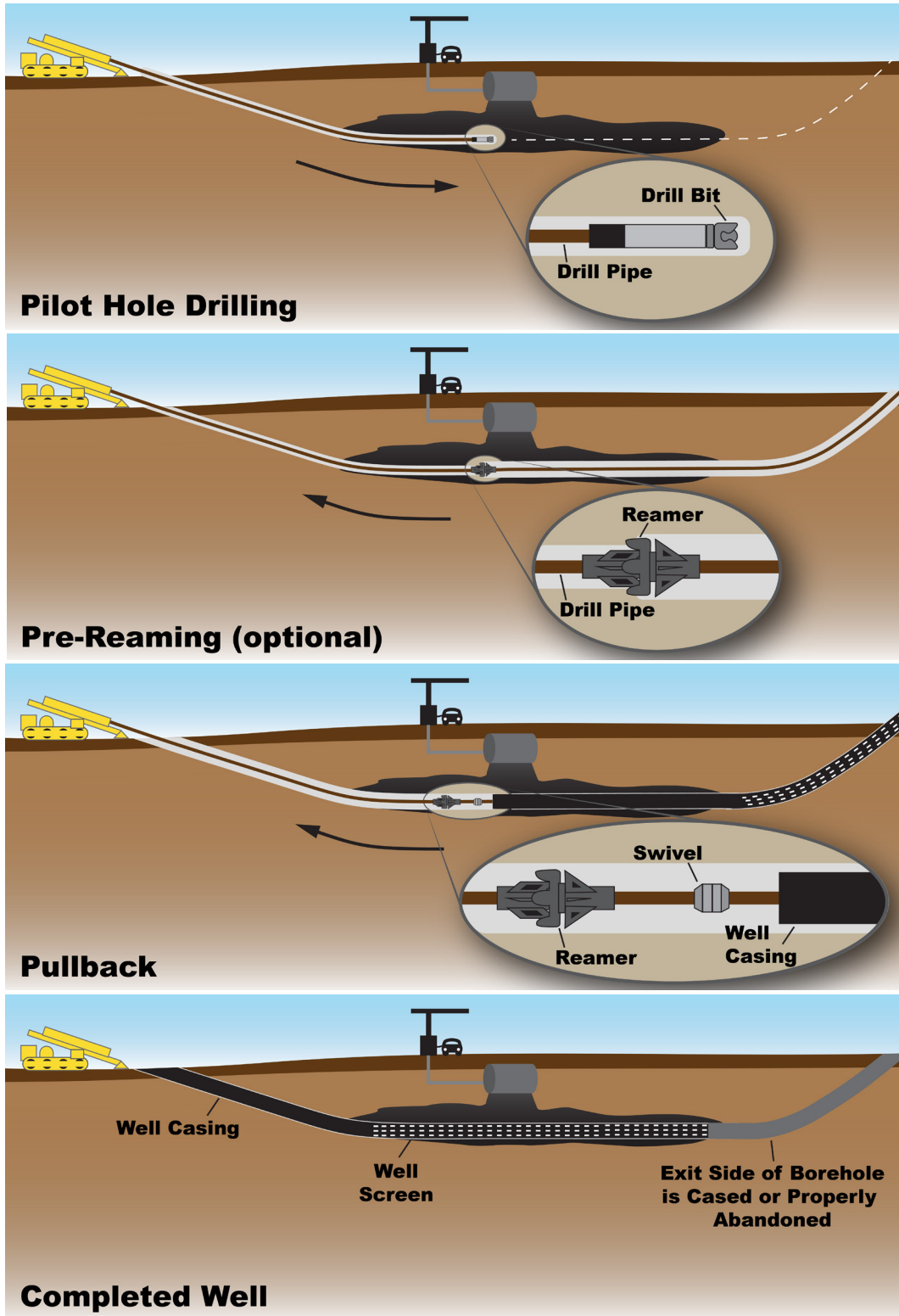
Exhibit A-17. Process Of Drilling Surface-To-Surface Well
