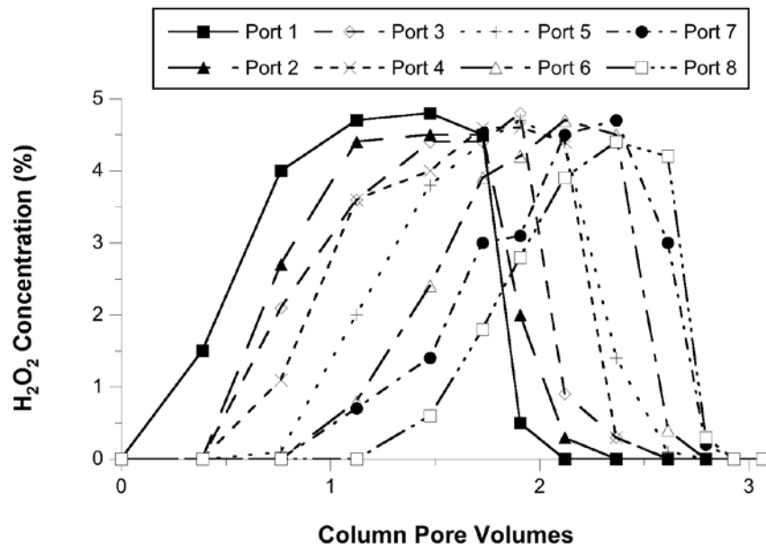
Figure 1-17. Concentration of 5% H 2 O 2 stabilized by 25 mM citrate at eight ports in a column of manganese-coated sand
